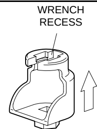
FIGURE 7 W-TYPE 6 SPRINKLER WRENCH
