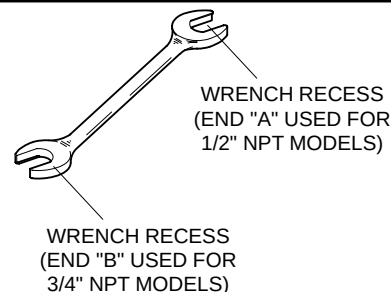
FIGURE 7 W-TYPE 6 SPRINKLER WRENCH
